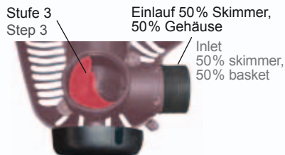
5 - stufig regulierbarer Skimmeranschluss 5-step adjustable skimmer connection
