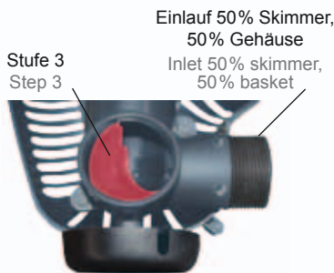
5 - stufig regulierbarer Skimmeranschluss 5-step adjustable skimmer connection
